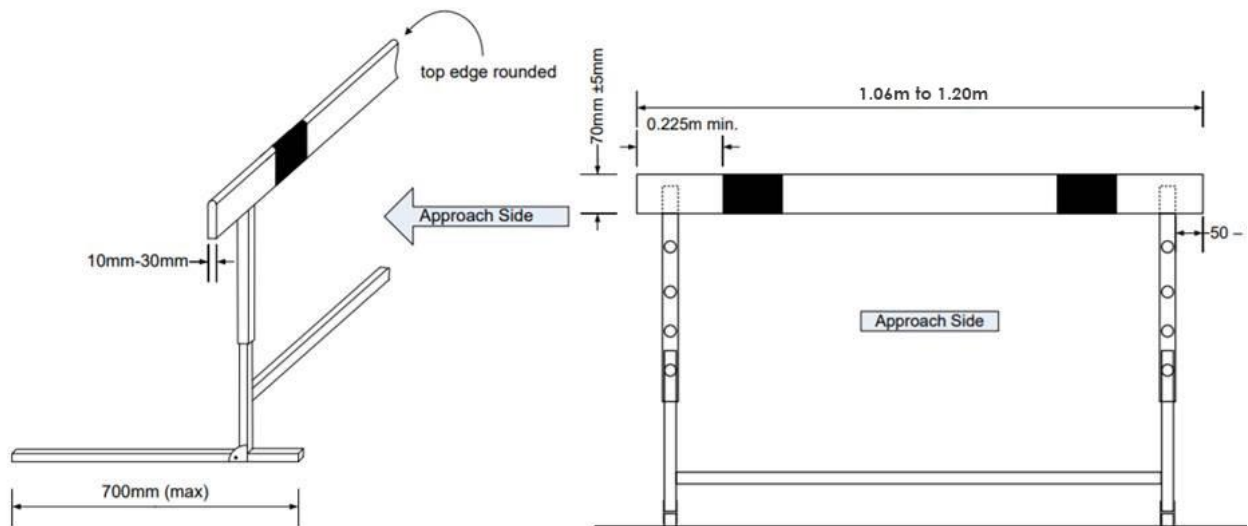
Collapsible Hurdle dimensions.
